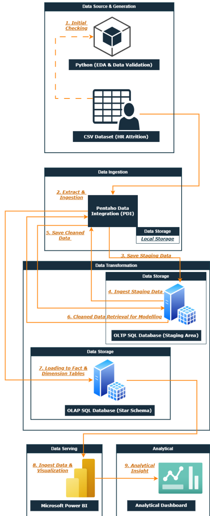
Fig. 4. Flowchart Research Framework
